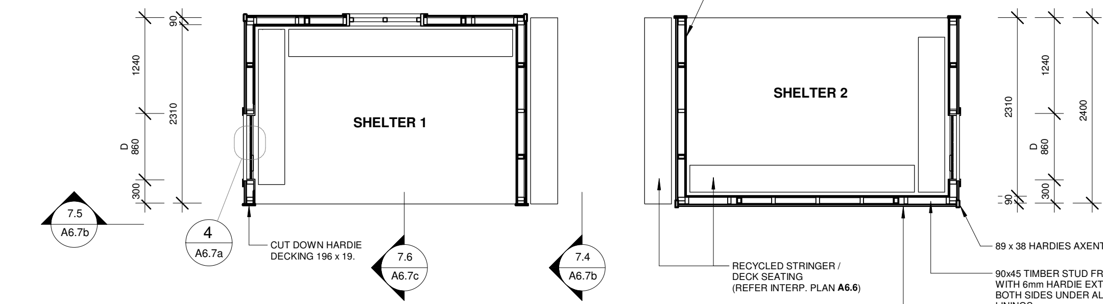
7.1 PLAN DETAIL 1:50
