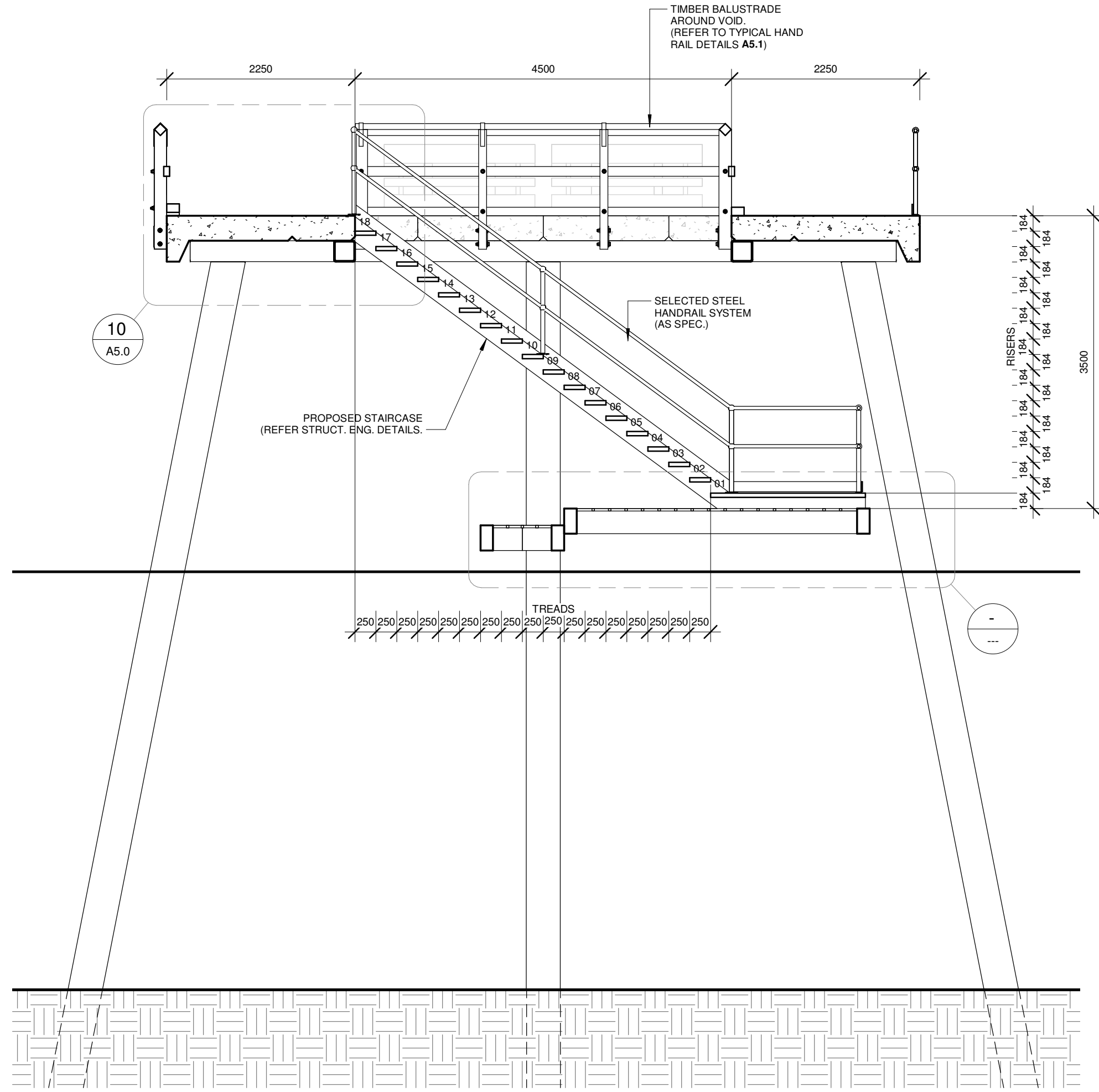
2 CROSS SECTION THROUGH PILE FRAME TYPE 4 A2.4 1 : 50
