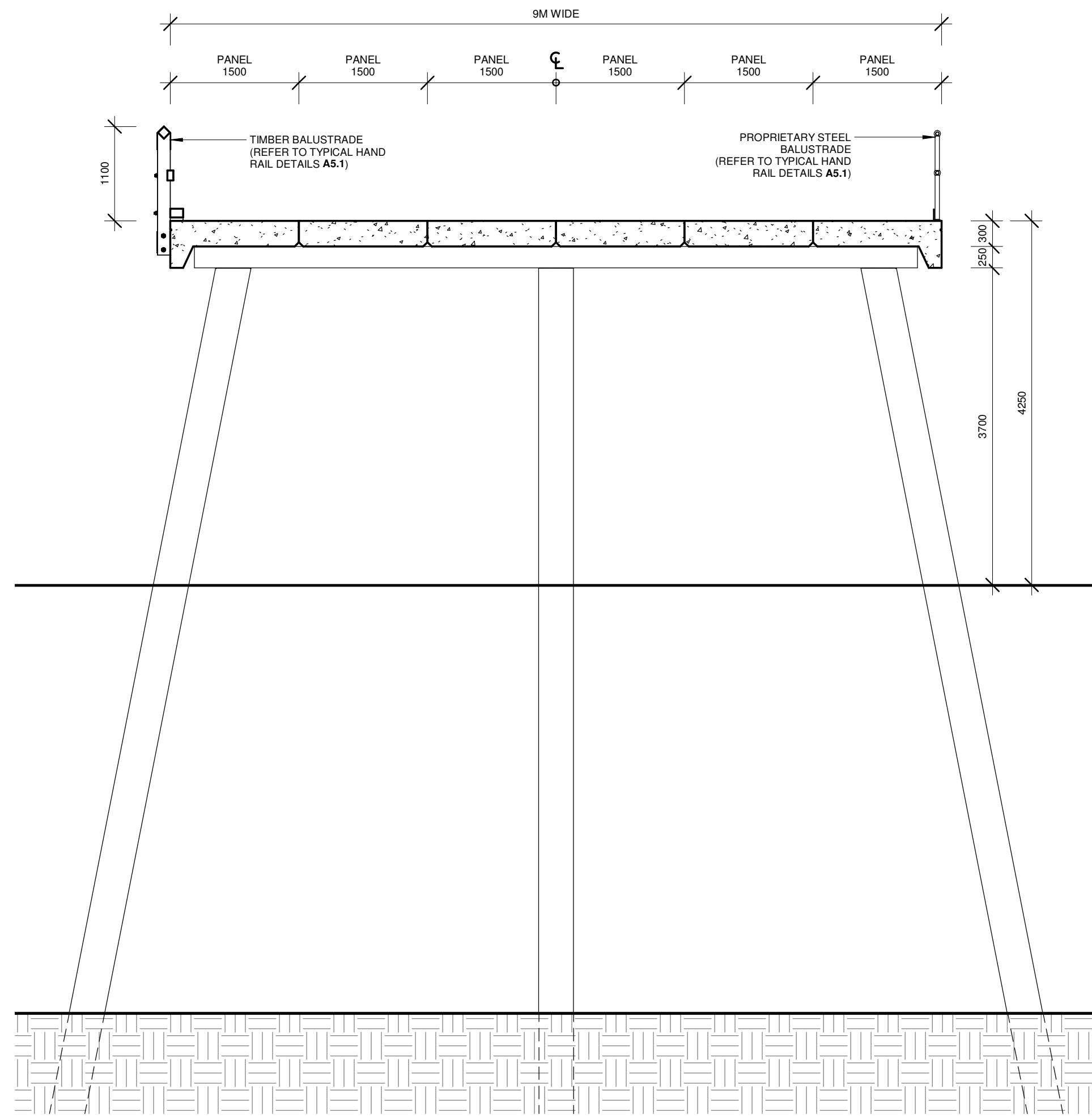
1 TYPICAL CROSS SECTION THROUGH PILE FRAME TYPE 4 A2.4 1 : 50
